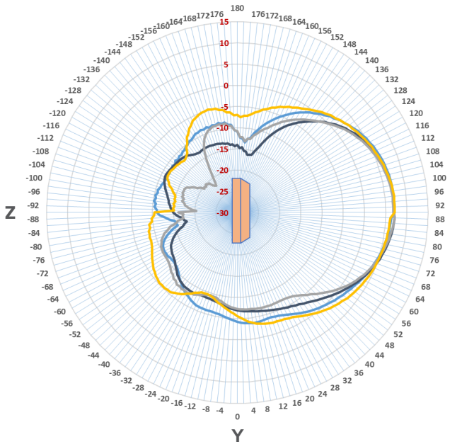
YZ Plane
