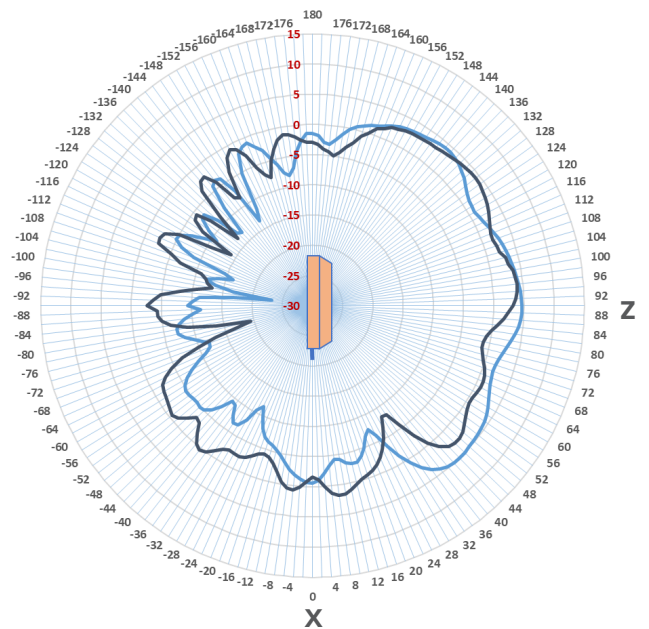
XZ Plane
