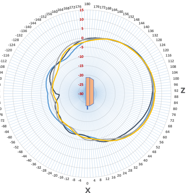
XZ Plane
